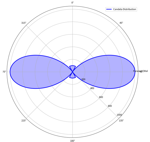
Photometric Polar Diagram Outdoor Wall Light 16W 5000K (1760 lm, 120° spread)
