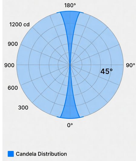
Photometric Polar Diagram - Outdoor Cylinder Up/Down Wall Light 18W 5000K (~1980 lm, 45° beam spread)
