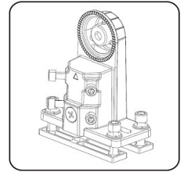
Universal (A+N TYPE)
