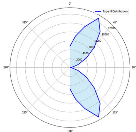
Photometric Polar Curve 240W LED Shoebox Area Light (36,000 lm, Type III)
